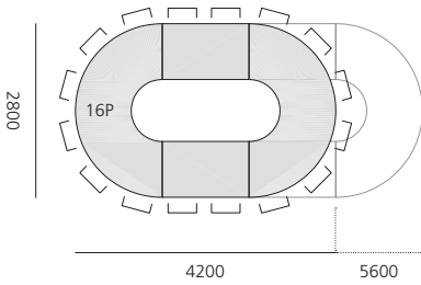
Flachoval - Ring
